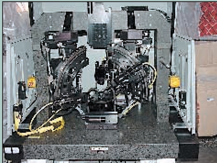
NEWPORT 4500 LASER WELDER
